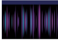
Shock Waves in Dusty Plasmas with Fast Particles
